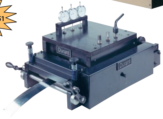
SS-10 Flat Stock Straightener
